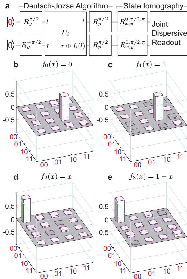
Figure 1: Implementation of Deutsch–Jozsa algorithm. a , Gate sequence solving the Deutsch–Jozsa problem. The two-qubit gates U_i encode the four functions of one bit to one bit, f_0(x) = 0 , f_1(x) = 1 , f_2(x) = x , and f_3(x) = 1 - x , as the transformations |l, r\rangle \rightarrow |l, r \oplus f_i(l)\rangle ( \oplus denotes addition modulo 2). The encoding unitaries are U_0 = I \otimes I , U_1 = I \otimes R_x^\pi , U_2 = (I \otimes R_y^{\pi/2} R_x^\pi) cU_{00} (I \otimes R_y^{\pi/2}) , and U_3 = (I \otimes R_y^{-\pi/2} R_x^\pi) cU_{11} (I \otimes R_y^{-\pi/2}) , respectively. b–e , Real part of the inferred density matrix \rho_{ml} of the algorithm output in the four cases (imaginary elements of \rho_{ml} are less than 0.05, 0.03, 0.05, 0.06, respectively). For the constant (balanced) functions f_0 and f_1 ( f_2 and f_3 ), \rho_{ml} reveals high fidelity to |1, 0\rangle ( |0, 0\rangle ), as expected. For the tomographs shown, the fidelity to the ideal output state is F = 0.94, 0.95, 0.92 , and 0.85 , respectively. Statistics for 8 runs of each of the four cases are given in Table 1 of the main text.
