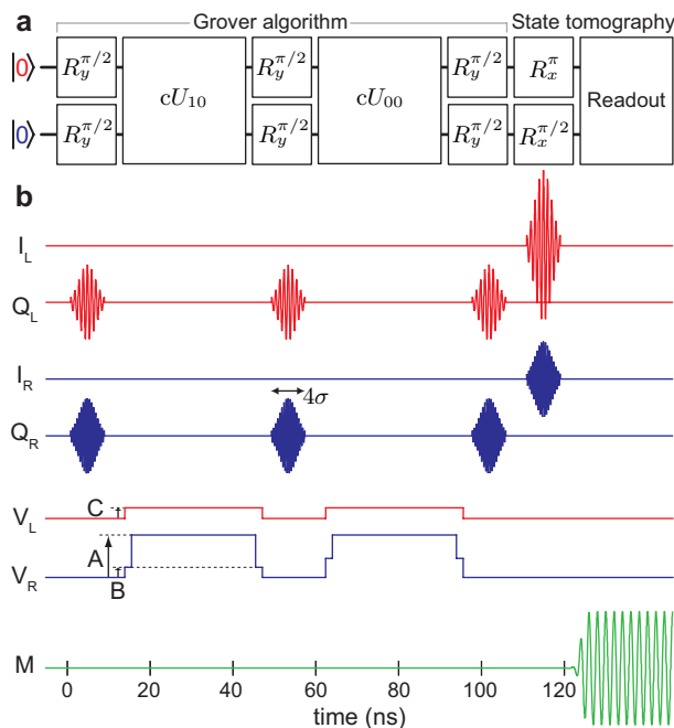
Figure 3: Microwave and flux pulses realizing the gates. a , An example sequence, executing the Grover search algorithm with oracle O = cU_{10} and measuring M_{13} = -\beta_1\sigma_z^L + \beta_2\sigma_y^R - \beta_{12}\sigma_z^L \otimes \sigma_y^R . b , Illustration of the microwave and flux pulses realizing the operations directly above. All microwave pulses implementing the x - and y -rotations have Gaussian envelopes, with standard deviation \sigma = 2 ns, truncated at \pm 2\sigma . The rotation axis is set using I-Q (vector) modulation (see Supplementary Fig. 2), and rotation angle is controlled by pulse amplitude. Flux pulses implementing C-Phase gates have three tuning parameters: the amplitude A of V_R , the amplitude B of 1 ns ledges at the beginning and end of the V_R -pulse, and the amplitude C of V_L . Pulse duration is fixed at 30 ns. A buffer of 5 ns is inserted between all microwave and flux pulses to avoid any overlap.
