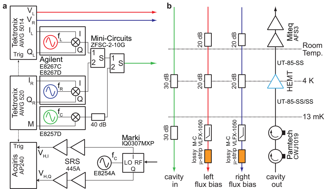
Figure 2: Experimental setup and wiring. a , Block diagram of room-temperature electronics. Arbitrary waveform generators, with 1 ns sampling rate and 10-bit resolution, produce voltages V_L and V_R directly applied to the flux-bias lines, the I-Q modulation envelopes for the microwave tones driving single-qubit x - and y -rotations, and the pulse that modulates the cavity measurement. On the output side, an I-Q mixer and a two-channel averager (2 ns, 8-bit sampling) complete the readout chain performing homodyne detection of the cavity quadratures. The arbitrary waveform generators, microwave synthesizers and acquisition card are clocked with a Rubidium frequency standard (SRS FS725, not shown). b , Schematic of microwave wiring inside the dilution refrigerator, showing heavily-attenuated input lines and an output chain with \sim 100 dB gain over 4–8 GHz.
