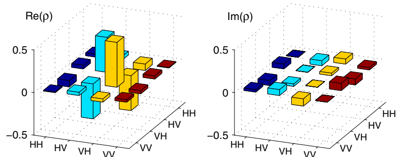
Fig. 3. State tomography. Reconstructed density matrix \rho for Alice’s and Bob’s nonlocal two-photon state, with tangle (36, 37) T = 0.68 \pm 0.04 , confirming the entanglement (37) of the widely separated photons, with linear entropy (37) 0.21 \pm 0.03 , and an optimal fidelity with a maximally entangled state F_{\text{opt}} = 0.91 \pm 0.01 . The measured state predicts a Bell parameter of S^{\text{tomo}} = 2.41 \pm 0.06 , which agrees with the directly measured value, and an optimal violation of S^{\text{opt}} = 2.54 \pm 0.06 for a rotated set of polarization measurements. The nonzero imaginary components are mainly due to polarization rotations resulting from imperfections in the alignment of Alice’s and Bob’s shared reference frame.
