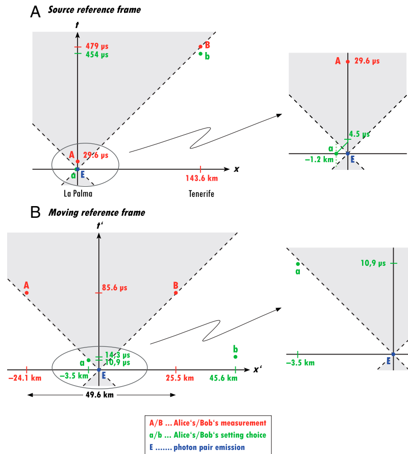
Fig. 2. Space-time diagrams. (A) Source reference frame. The forward (backward) light cone of the photon-pair emission event E, shaded in gray, contains all space-time events which can be causally influenced by E (can causally influence E). Alice's random setting choices (indicated by small green dots in the zoomed part of A), each applied for a 1- \mu s interval, were transmitted over a 1.2-km classical link (green line), which took 4.5 \mu s (3.9 \mu s classical rf link, 0.6- \mu s electronics). This signal was electronically delayed by 24.6 \mu s, so that the choice event a, corresponding to a given measurement A, occurred simultaneously within a time window of \pm 0.5 \mu s with the emission event E, i.e., E occurred on average in the middle of the 1- \mu s setting interval. The choice and emission events were therefore space-like separated. The same electronic delay (24.6 \mu s) was applied to Bob's choice b, so that it was also space-like separated from the source. (B) Moving reference frame. From the perspective of an observer moving at a speed of 0.938c parallel to the direction from La Palma (Alice) to Tenerife (Bob), the measurement events, A and B, occur simultaneously with the emission event approximately in the middle of the two. The locality and the freedom-of-choice loopholes are closed in the source reference frame, and because space-like separation is invariant under Lorentz transformations, they are closed in all reference frames. In the diagrams above, the total uncertainty of the event times is below the size of the illustrated points (see Materials and Methods ).
